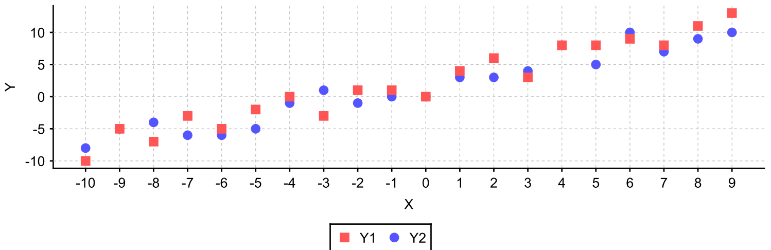
Scatter chart
